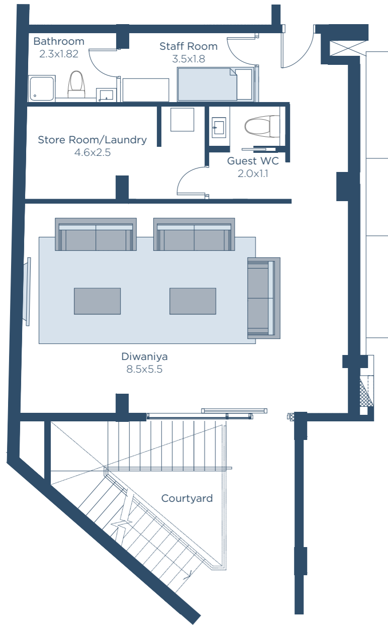
Basement Floor Area 92.5 sqm
